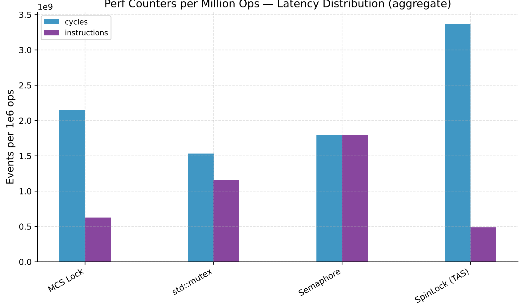
Perf Counters per Million Ops — Latency Distribution (aggregate)
